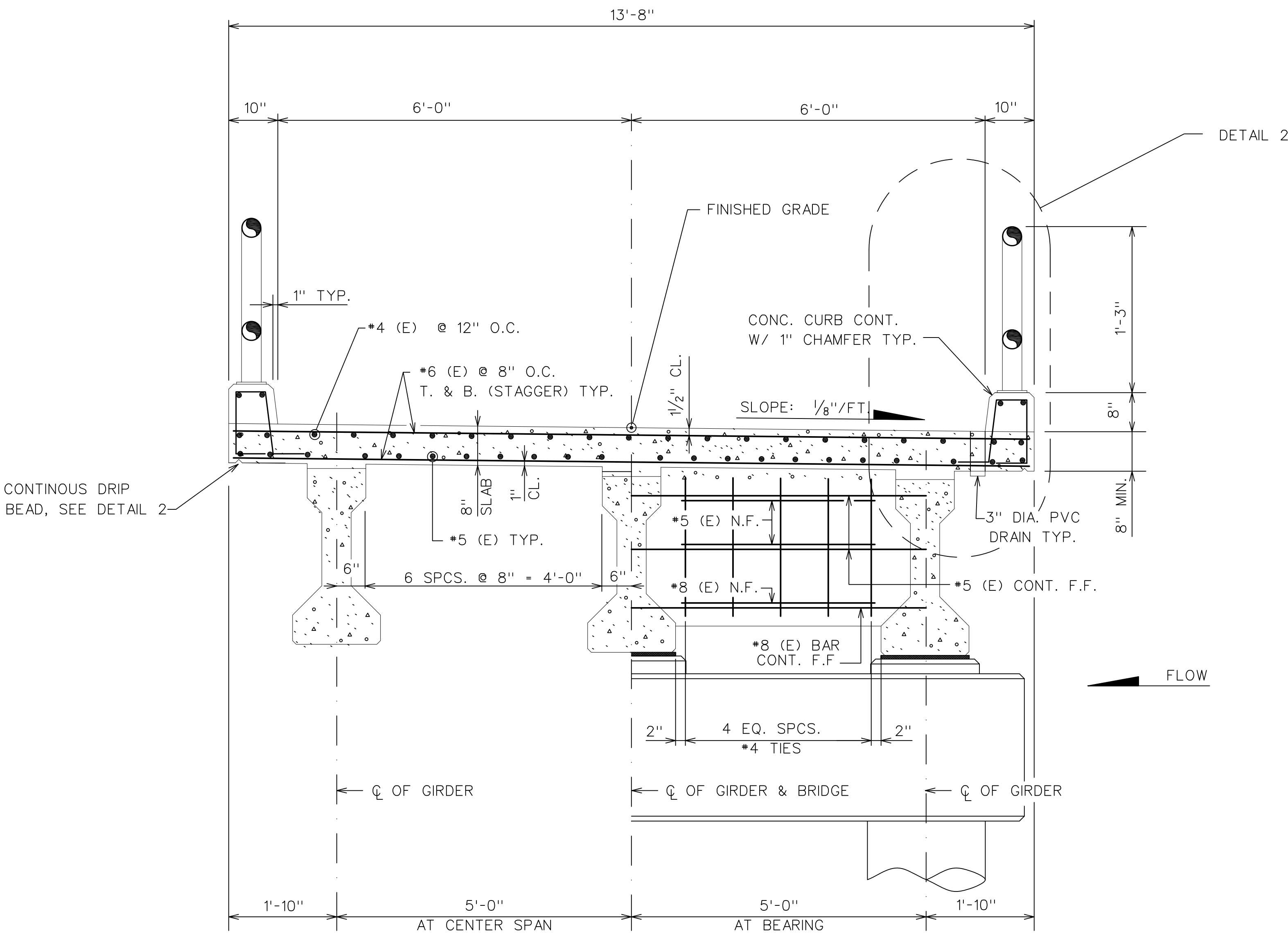
TYPICAL CROSS SECTION SCALE: 3/4" = 1'-0" (LOOKING TOWARD BANK)
