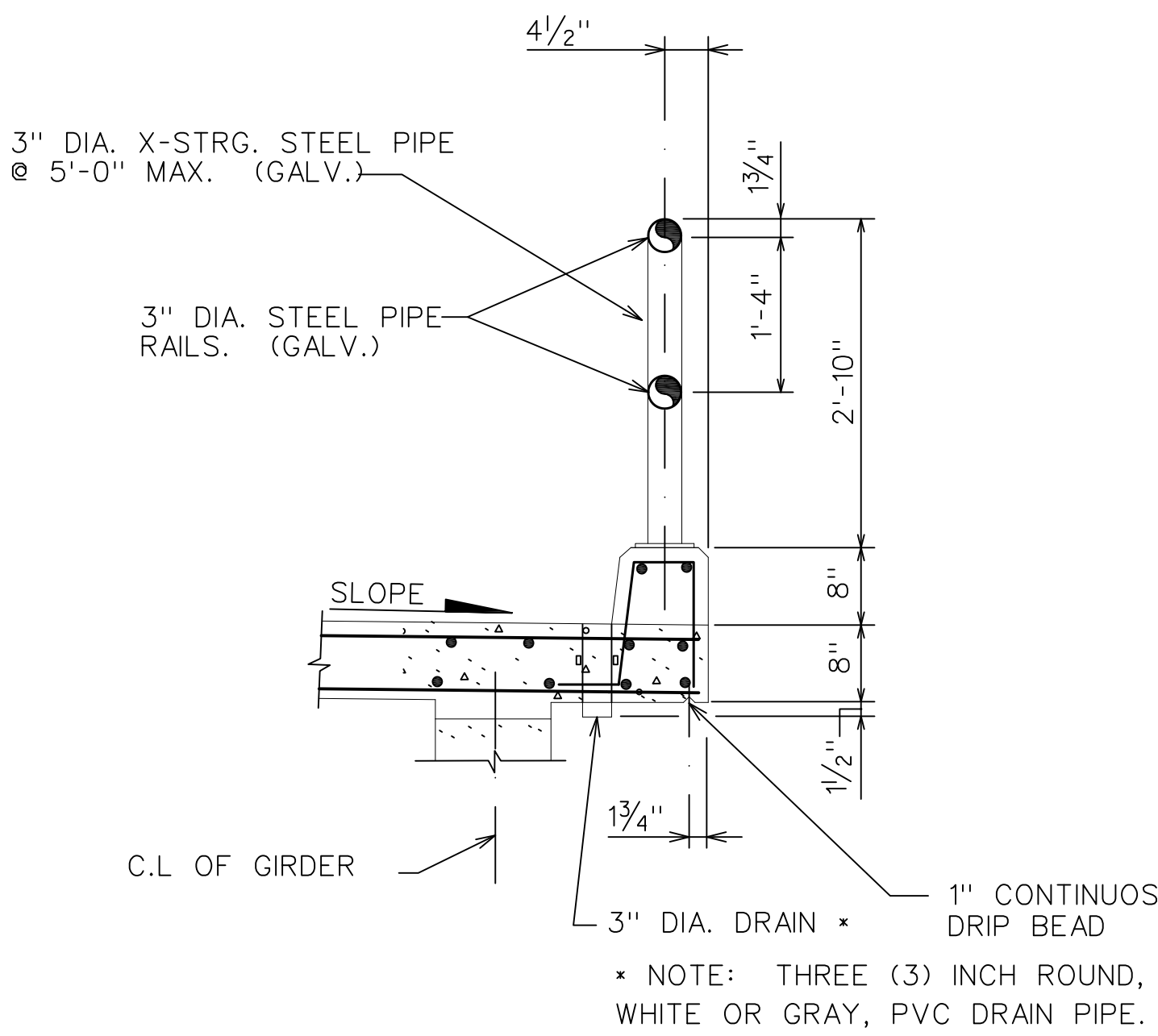
GUARDRAIL DETAIL 2 NOT TO SCALE
