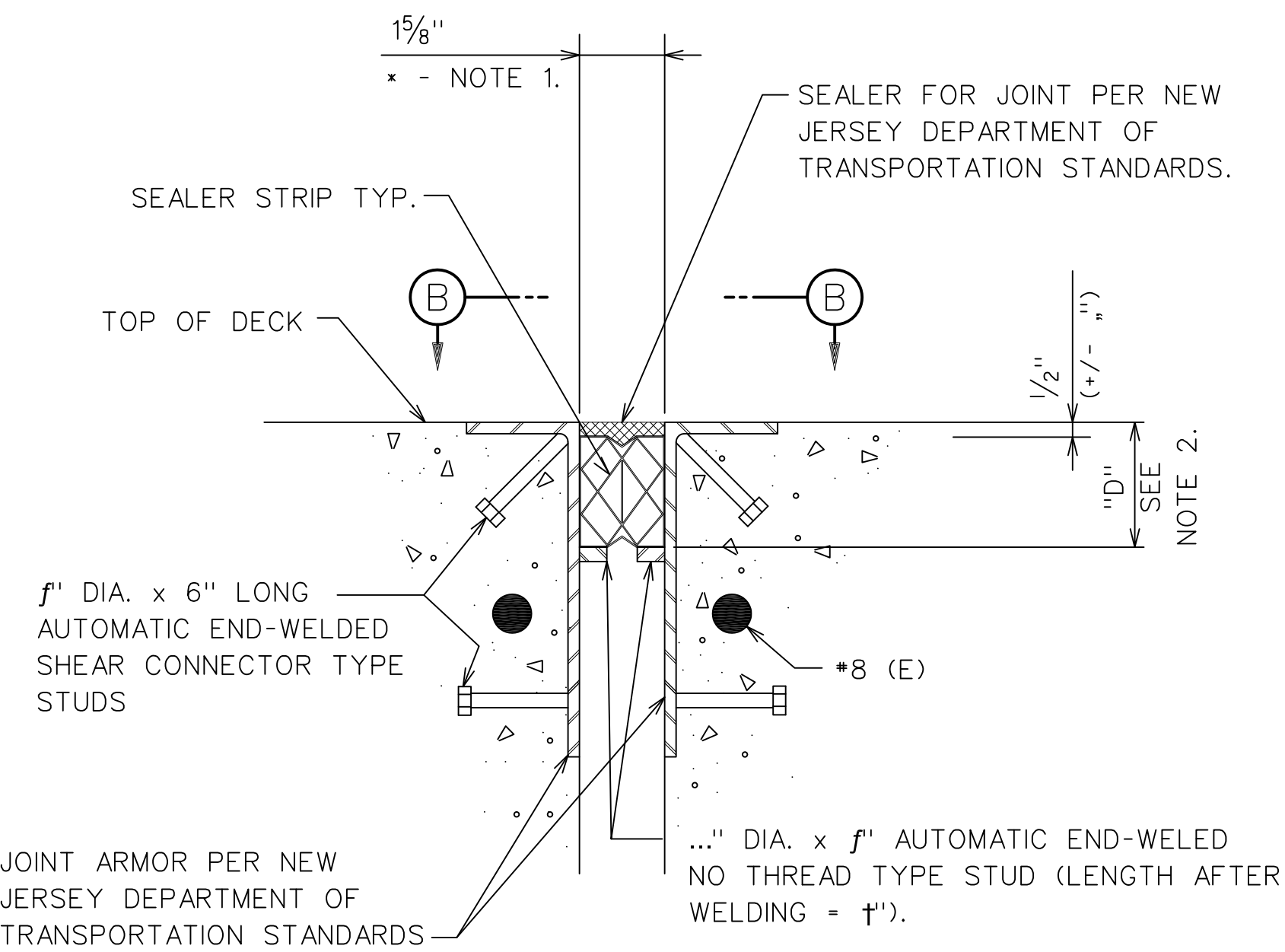
DETAIL 1 NOT TO SCALE
